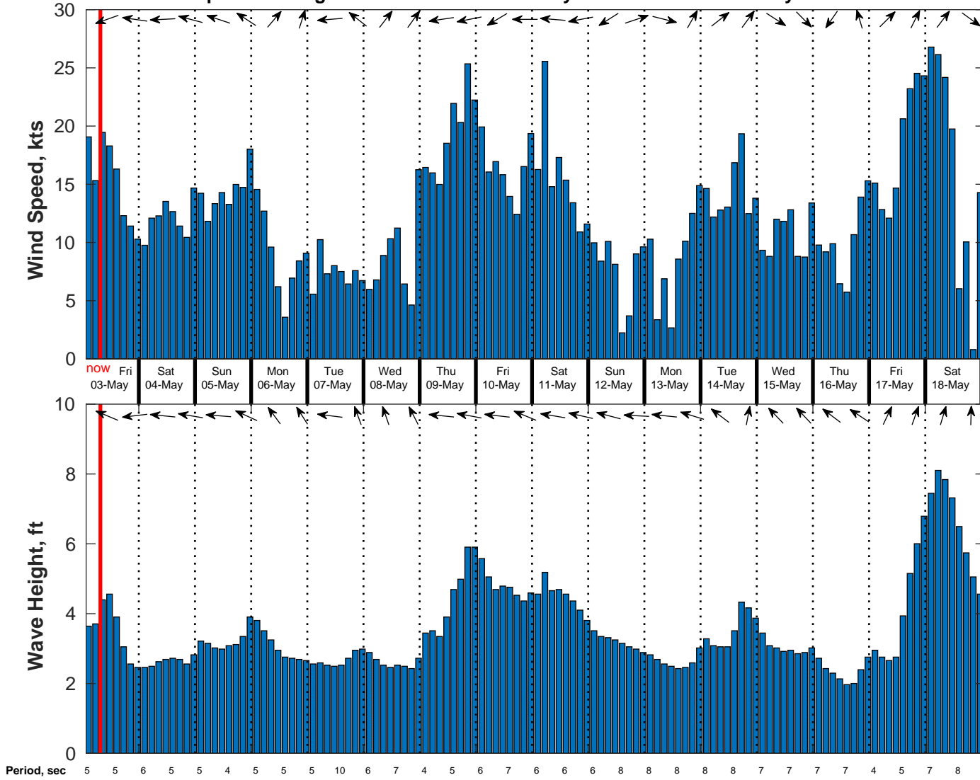
Wind & Wave Forecast for Equinor NY Bight OCS-A 0512 from 03-May-2024 01:00:00 to 19-May-2024 01:00:00
